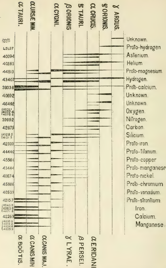
FIG. 27.—Map of chemical substances present in stars of different temperatures.
